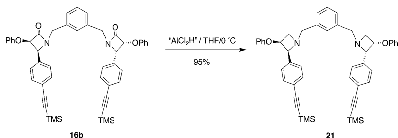
Scheme 4. Synthesis of azetidine derivative 21 .
