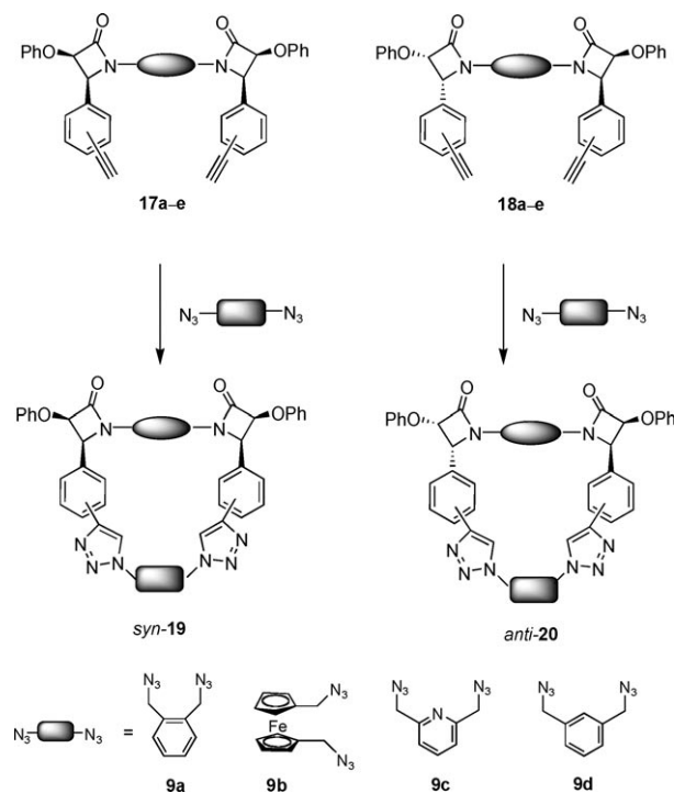
Scheme 5. Synthesis of macrocycles 19 and 20 .
