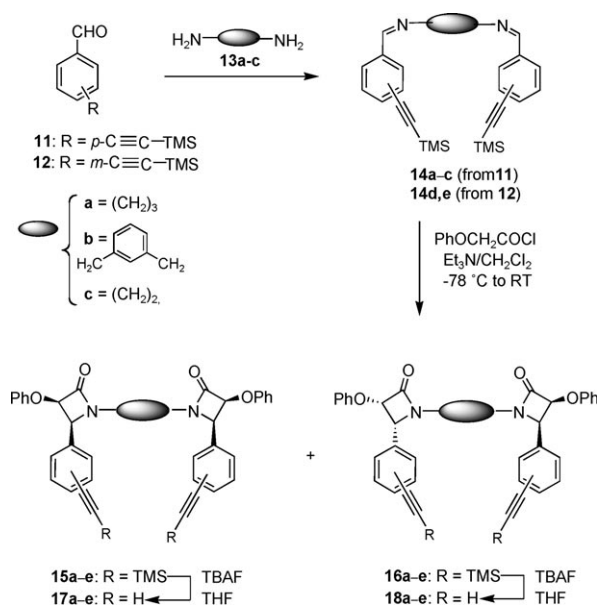
Scheme 3. Synthesis of the starting bis-alkynyl-β-lactams.
