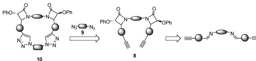
Scheme 2. Synthetic planning for 10 .
