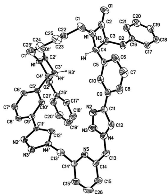
Figure 3. ORTEP plot of 19n with 25 % probability. Hydrogen atoms are omitted for clarity, with an exception made for H3, H4, H3', and H4' bonded to the chiral carbon atoms.
