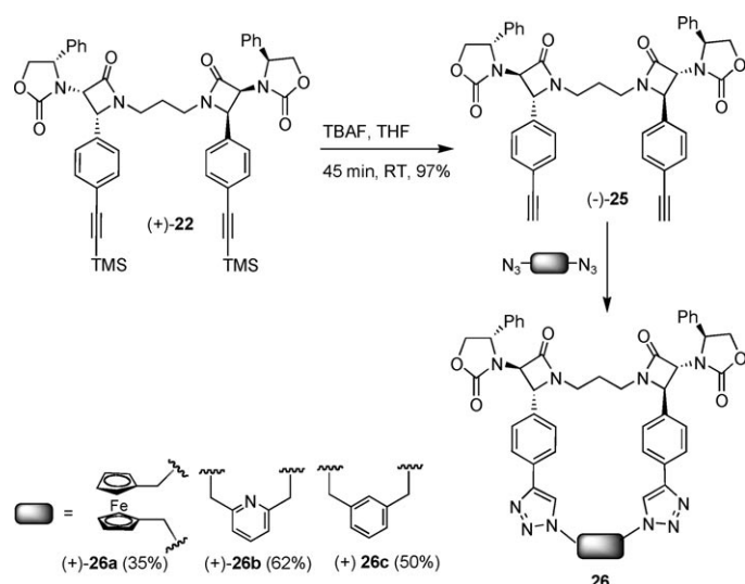
Scheme 7. Synthesis of enantiopure macrocyclic β-lactam cavities (+)-26.
