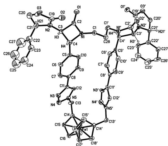
Figure 4. ORTEP plot of (+)-26a with 25% probability. Hydrogen atoms are omitted for clarity, with an exception made for H3, H4, H3', and H4' bonded to the chiral carbon atoms.
