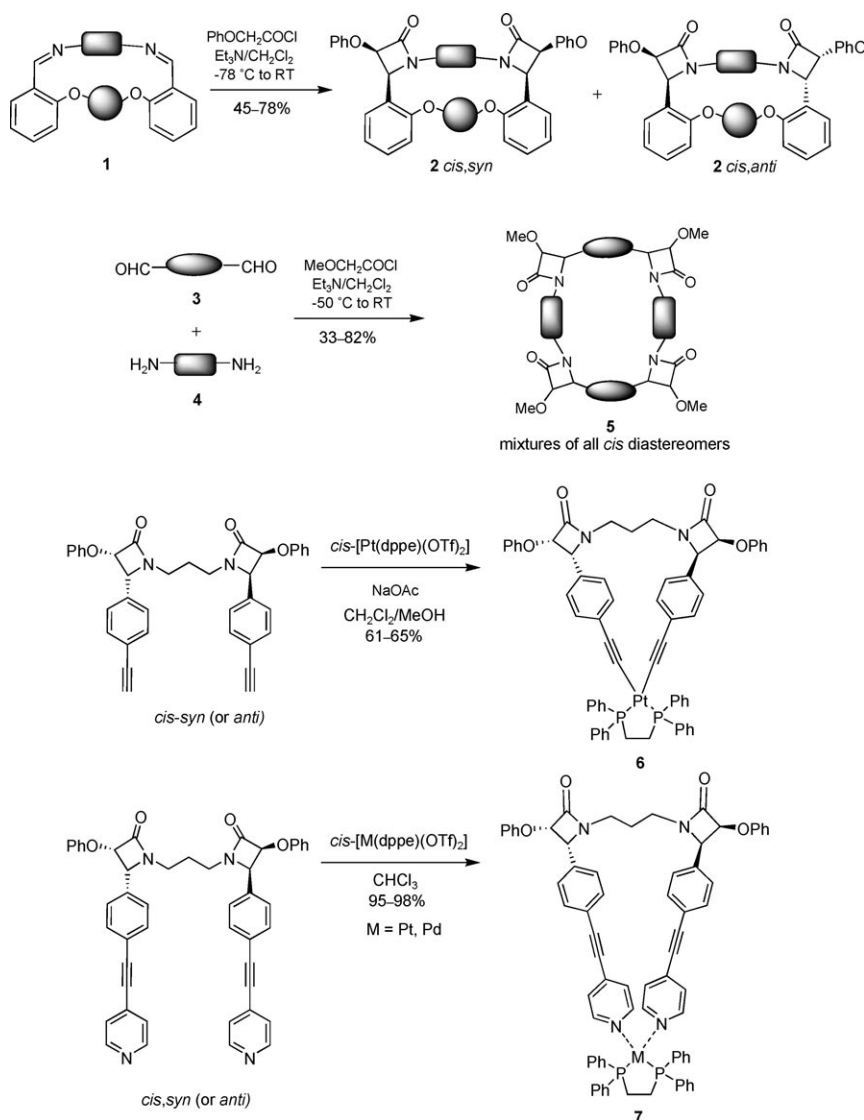
Scheme 1. A summary of the synthetic approaches used to build macrocyclic structures embedding 2-azetidinone rings (OTf = trifluoromethanesulfonate, dppe = 1,2-bis(diphenylphosphino)ethane).
