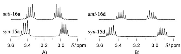
Figure 1. 1 H NMR spectra for compounds A) anti - 16a and syn - 15a , and B) anti - 16d and syn - 15d .
