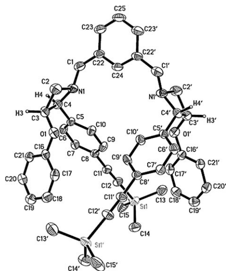
Figure 2. ORTEP plot of 21 with 25 % probability. Hydrogen atoms are omitted for clarity, with an exception made for H3, H4, H3', and H4' bonded to the chiral carbon atoms. The asymmetric unit is one half of the molecule.
