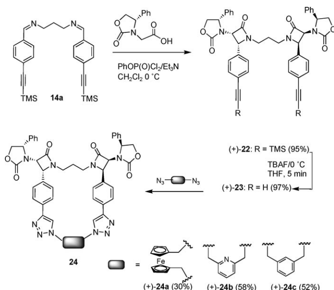
Scheme 6. Synthesis of enantiomerically pure macrocyclic bis- \beta -lactams (+)- 24a-c .
